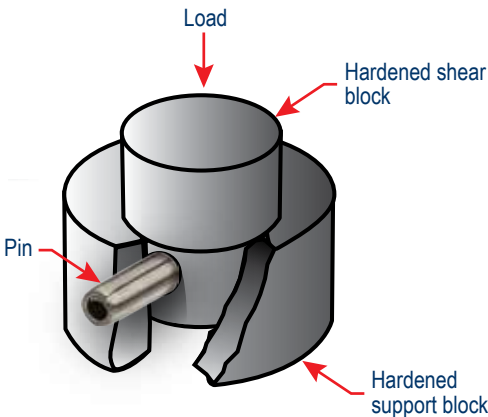
Shear test performed in a fixture per ISO 8749
